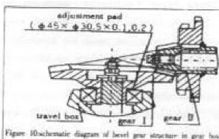
Figure 10: schematic diagram of bevel gear structure in gear box
