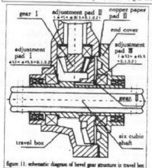
Figure 11: schematic diagram of bevel gear structure in travel box
